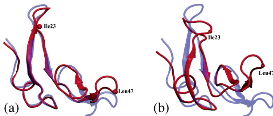
FIGURE 4: Comparison of the structures in the simulations of N-WT. (a) Superimposed structures between the initial structure of N-WT (Figure 1b) and the final one in S^{\text{MD}}_{\text{N-WT}} . (b) Initial structure of N-WT and the final one in S^{\text{ACM2MD}}_{\text{N-WT}} . Backbone atoms between residues 9–42 were used for the least-squares fit. The initial structure is colored light blue and the final structure solid red. The two residues, Ile23 and Leu47, are indicated by spheres.
