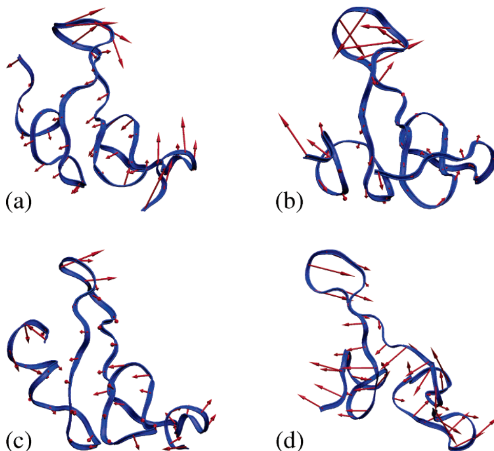
FIGURE 8: Essential dynamics analysis (EDA) of the EGF simulations. (a) N-WT, (b) EGF-II, (c) n-S9C, and (d) N-S9C. For each simulation of S_X^{ACM2MD} , C_\alpha atoms were used to perform EDA from the last 10 ns. The ribbons structure in blue is the configuration in the trajectory (20–30 ns) that has the most negative or positive projection on the first essential mode, and the red arrows indicate the motions of the C_\alpha atoms along this mode.
