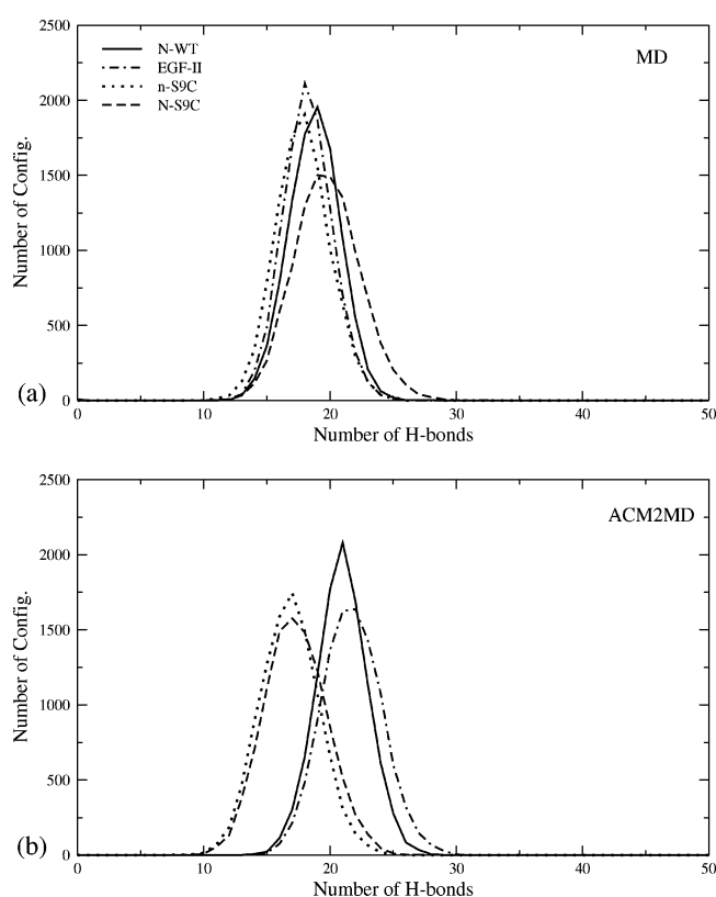
FIGURE 5: Distributions of the number of hydrogen bonds in the simulations of N-WT, EGF-II, and the two S9C isomers. (a) The last 10 ns (10,000 configurations) in each simulation of S^{\text{MD}}_{\text{X}} were used. (b) The last 10 ns (10,000 configurations) in each simulation of S^{\text{ACM2MD}}_{\text{X}} were used. Only the hydrogen bonds within the loops and between them were counted. The criteria for a hydrogen bond are a maximal distance of 0.25 nm between hydrogen–acceptor and a maximal 60^\circ for the angle donor–hydrogen–acceptor.
